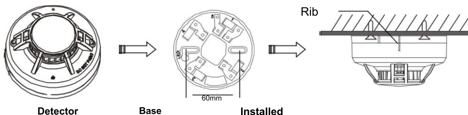
Figure 3. Install the detector
