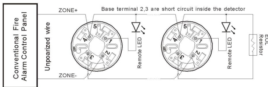
Figure 2. Typical wiring diagram
